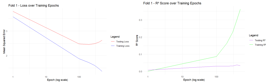
Figure 3. Loss over 400 epochs (log scale) of training and testing data for MLP model in fold 1.
