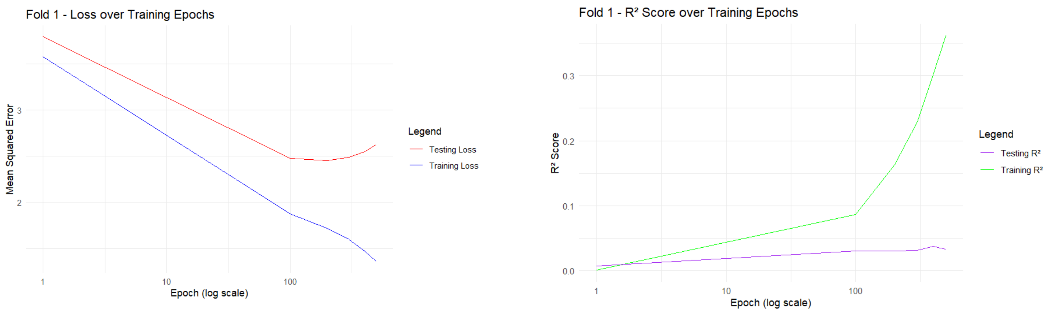
Figure 6: Loss and R 2 over 400 epochs of training and testing data for MLP model.
