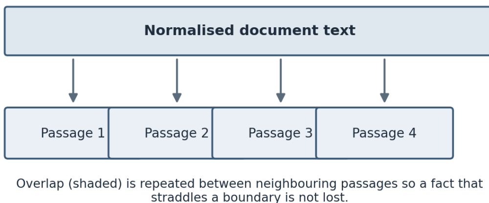
Figure 1. Chunking with overlap. A normalised document is split into passages of up to about 900 characters, with roughly 160 characters repeated between neighbours (shaded) so a fact that spans a boundary is not lost.
