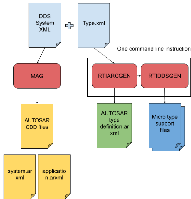
Figure 3.7: Workflow for converting XML files into AUTOSAR application code
