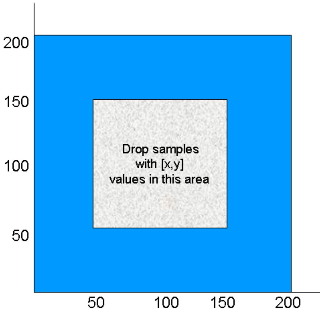
Figure 3.5: Filtering Example
