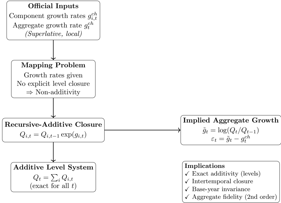
Fig. 1 RA closure: from superlative growth primitives to an exactly additive intertemporal level system.
