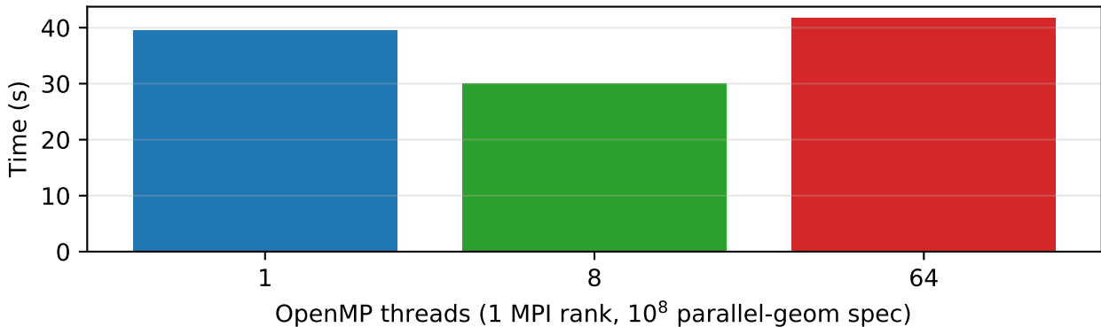
Compute-heavy neighbor loop: thread scaling (same expansions/cost)
