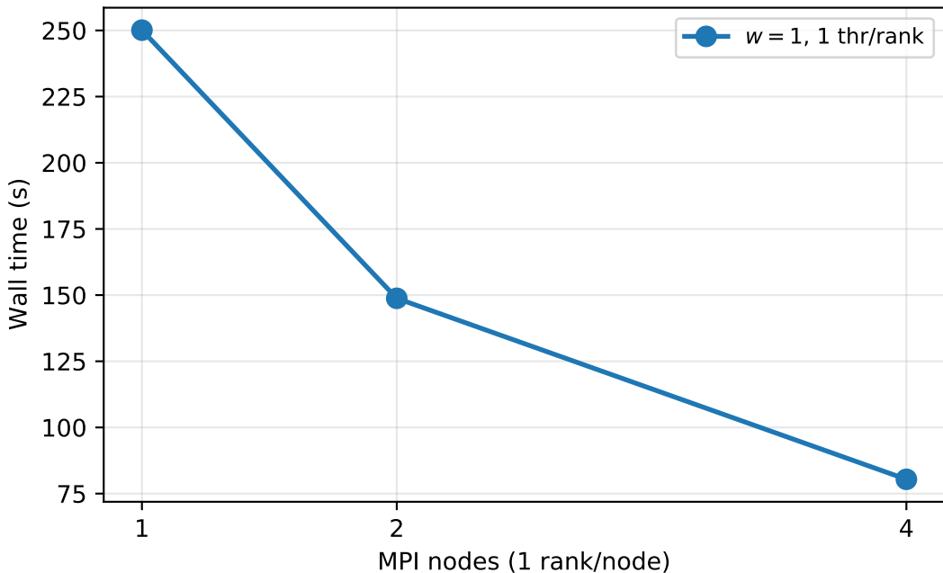
Strong scaling: geom recommender medium 10^9
