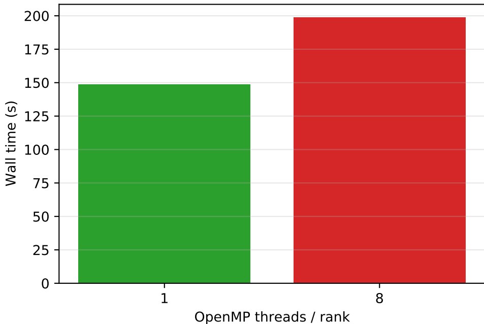
OpenMP at 2 nodes (geom medium 10^9 , w = 1 )
