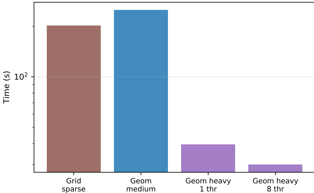
Neighbor-generation cost (1 node, 1 MPI rank)
