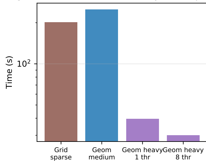
(4) Neighbor cost (1n, 1 rank; heavy = 10^8 parallel sp)
