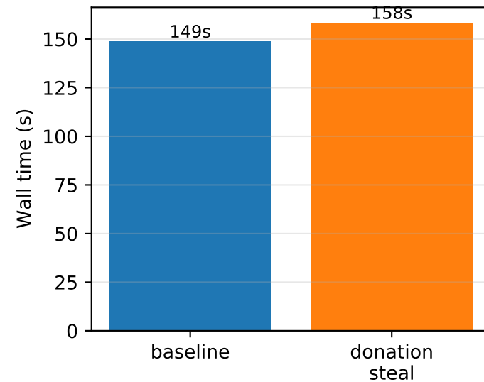
(6) Load balance: baseline vs steal (2n, 1 thr, geom medium w = 1 )
