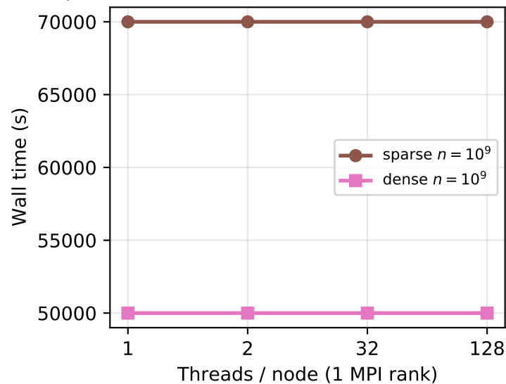
(5) Sparse vs dense grid, w = 5 , 1 node
