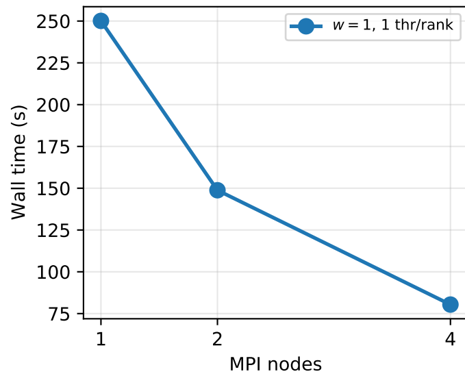
(1) Strong scaling: geom medium 10^9 , w = 1
