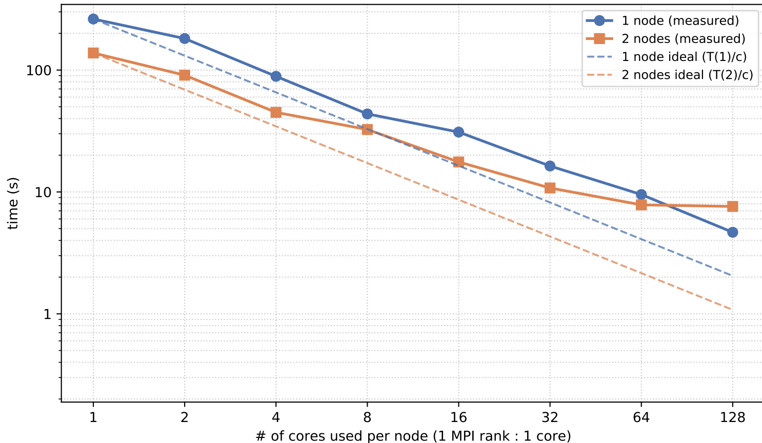
Geom recommender medium n=1e9 , w=1 — MPI scaling
