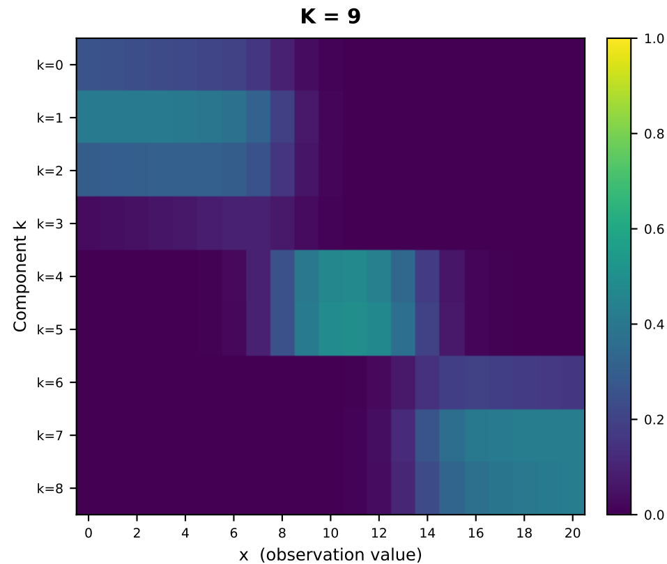
M_K(k, i) = q(c = k \mid x = i - 1, \pi, \theta) Final EM iteration responsibilities for each K
