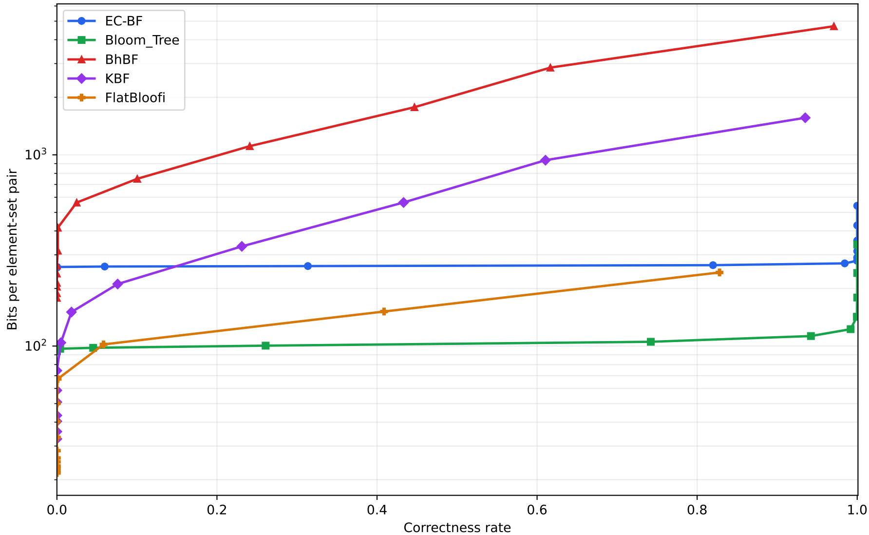
Correctness Rate vs Space
