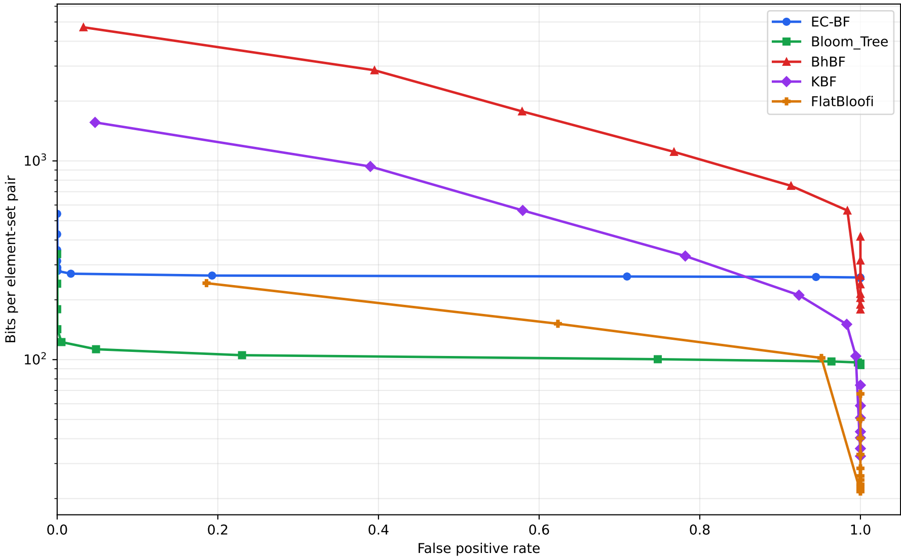
False Positive Rate vs Space
