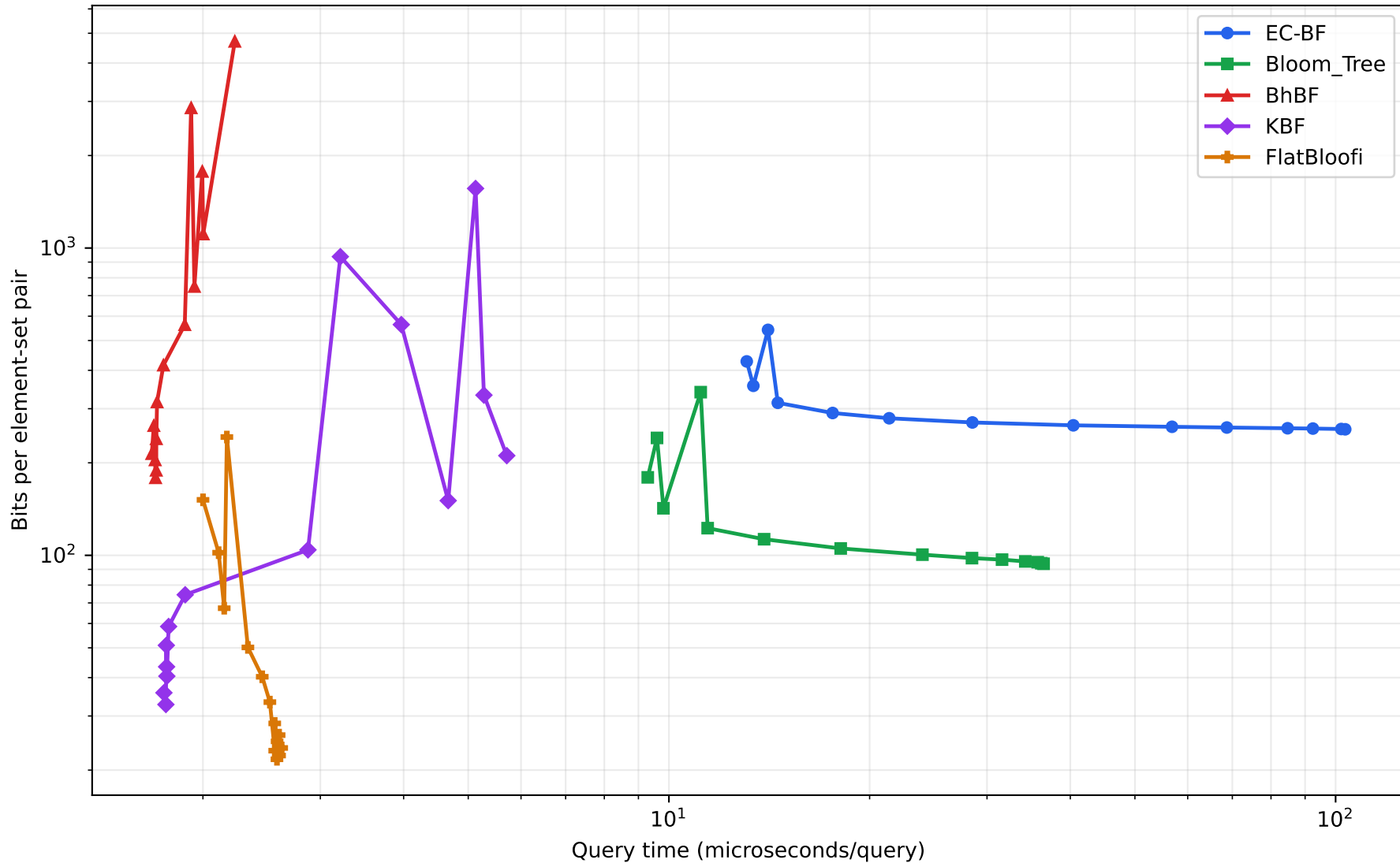
Query Speed vs Space
