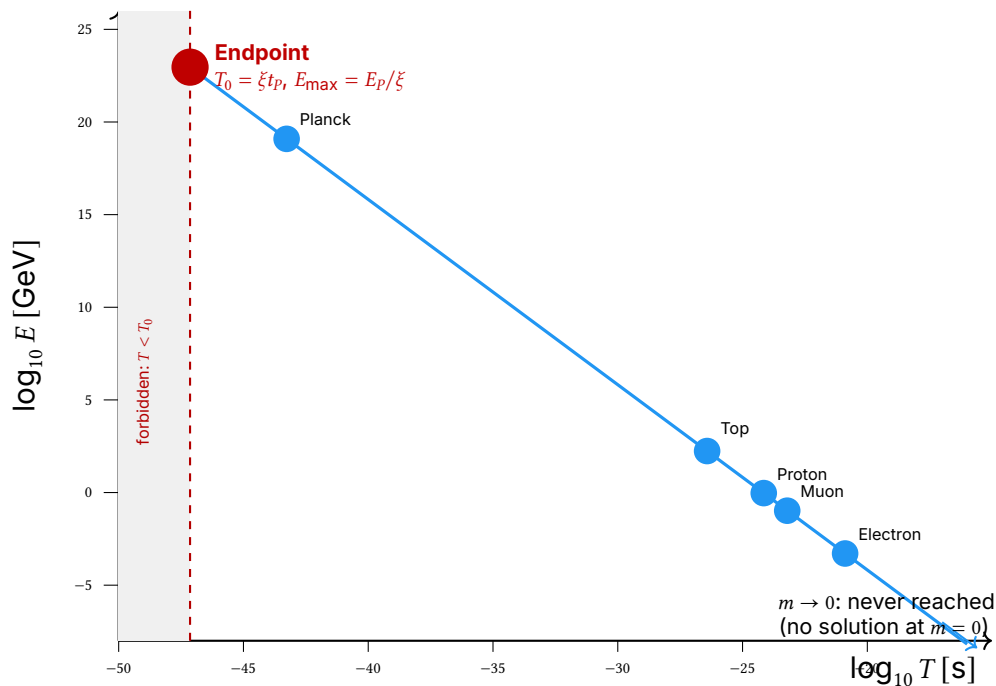
Figure 1: The relation T \cdot E = 1 (in SI: T \cdot E = \hbar ) in doubly logarithmic coordinates: a straight line of slope -1 . All elementary excitations lie exactly on it — none is privileged, and the line has no middle . Exactly one point is distinguished: the endpoint (T_0, E_{\max}) = (\xi t_p, E_p/\xi) , where the curve stops — the wall that follows from \xi . At the other end it continues as an asymptote and never arrives ( T \cdot m = 1 has no solution at m = 0 ). The two edges are therefore of different kinds: on the left an attained endpoint, on the right an unreachable limit. What is plotted are scales (energy per excitation), not total masses; macroscopic bodies do not belong on this axis.
