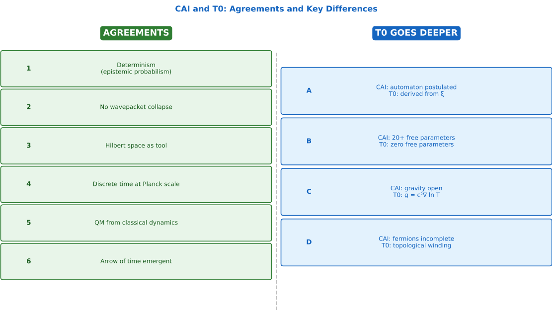
Figure Q.6: Agreements (green, left) and fundamental differences (blue, right) between the CAI and T0 theory.
