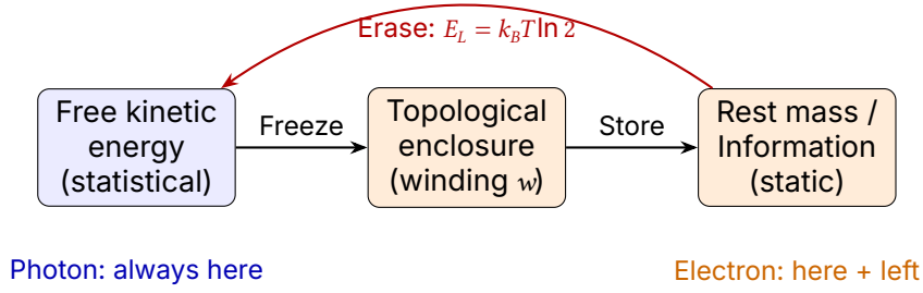
Figure ag.1: Energy division in FFGT. Free kinetic energy (blue) can be transferred into static mass/information (orange) through topological enclosure. Erasure (red arrow) releases the frozen energy as heat – Landauer’s principle. The photon remains permanently in the kinetic sector.
