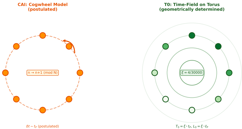
Figure S.2: Left: CAI cogwheel with N = 8 discrete states (postulated). Right: T0 time field on geometric torus, lattice spacing L_0 = \xi \cdot \ell_P (derived).
