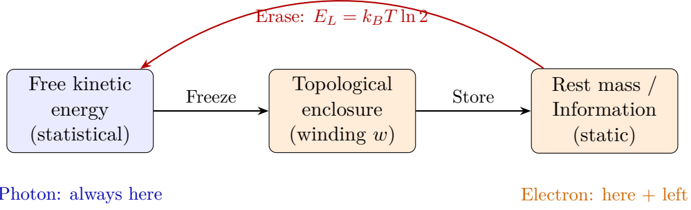
Figure 1: Energy division in FFGFT. Free kinetic energy (blue) can be transferred into static mass/information (orange) through topological enclosure. Erasure (red arrow) releases the frozen energy as heat – Landauer’s principle. The photon remains permanently in the kinetic sector.
