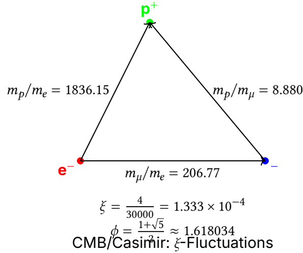
Figure 2.1: Fundamental Mass Triangle of the e-p- \mu System (extended by cosmological \xi -effects)
