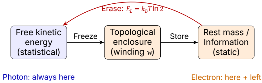
Figure ag.1: Energy division in FFGFT. Free kinetic energy (blue) can be transferred into static mass/information (orange) through topological enclosure. Erasure (red arrow) releases the frozen energy as heat – Landauer’s principle. The photon remains permanently in the kinetic sector.
