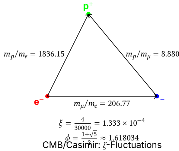
Figure 1: Fundamental Mass Triangle of the e-p- \mu System (extended by cosmological \xi -effects)
