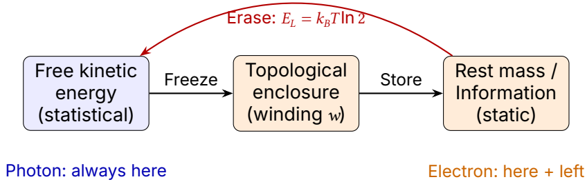
Figure af.1: Energy division in FFGFT. Free kinetic energy (blue) can be transferred into static mass/information (orange) through topological enclosure. Erasure (red arrow) releases the frozen energy as heat – Landauer’s principle. The photon remains permanently in the kinetic sector.
