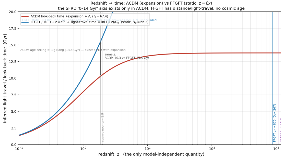
Figure 0.1: Redshift \rightarrow time is model-dependent. \Lambda CDM look-back (red, expansion +\Lambda ) saturates at the Big Bang ceiling 13,8 Gyr; FFGFT (blue, static, 1+z=e^{\xi x} ) gives an unbounded light-travel time \ln(1+z)/H_0 with no Big Bang. At cosmic noon ( z \approx 1,9 ): \Lambda CDM 10,3 vs. FFGFT 15,5 Gyr. Recombination: \Lambda CDM z_* \approx 1100 , FFGFT z_* \approx 875 (Doc. 267).
