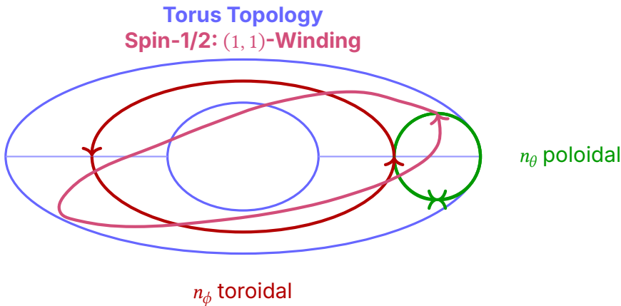
Figure 1: Spin-1/2 as topological winding on a torus (top view).
