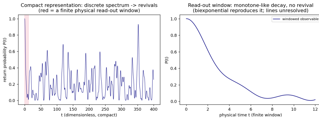
Figure S.1: Read-out as a non-invertible projection. Left: on the compact representation the discrete spectrum produces revivals (back-flow \gg 0 ); the red band marks a finite physical read-out window. Right: inside the window the observable decays without revival and the discrete lines are unresolved.
