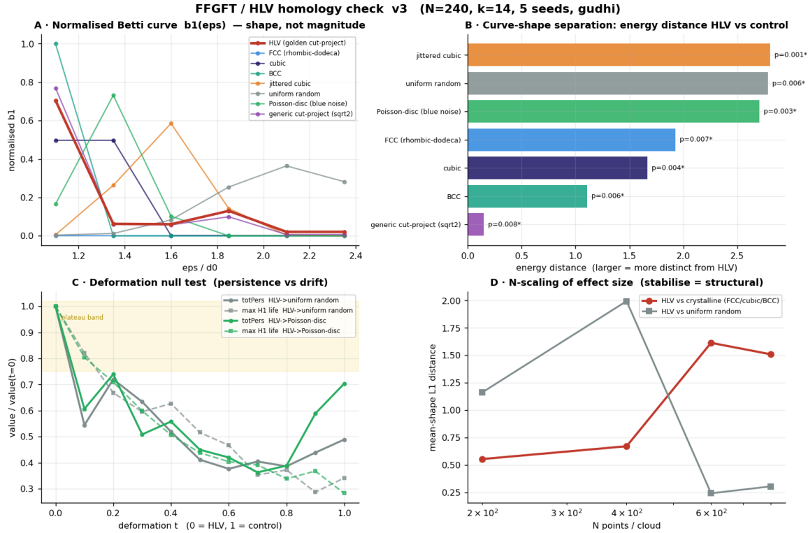
Figure L.1: Four-panel overview from the companion script (v3). A: normalised Betti curves b_1(\epsilon) – shape, not magnitude. B: curve-shape energy distance HLV vs. controls. C: deformation null test (total persistence and, with gudhi, longest H_1 lifetime). D: N-scaling of the effect size (stable = structural). Finite diagnostic; no claim about physical spacetime microstructure.
