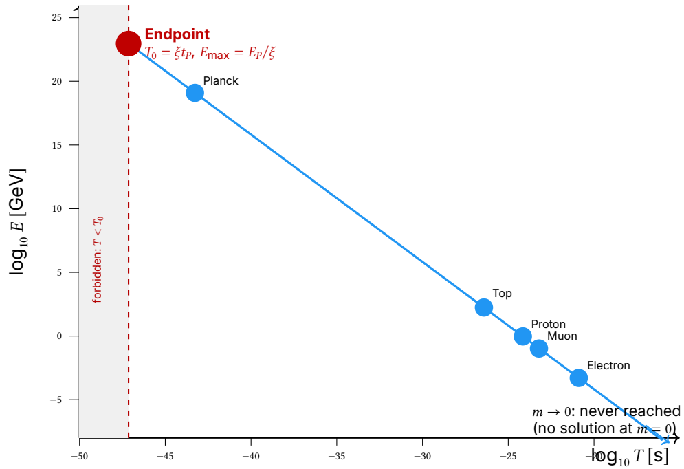
Figure ao.1: The relation T \cdot E = 1 (in SI: T \cdot E = \hbar ) in doubly logarithmic coordinates: a straight line of slope -1 . All elementary excitations lie exactly on it — none is privileged, and the line has no middle . Exactly one point is distinguished: the endpoint (T_0, E_{\max}) = (\xi t_P, E_P/\xi) , where the curve stops — the wall that follows from \xi . At the other end it continues as an asymptote and never arrives ( T \cdot m = 1 has no solution at m = 0 ). The two edges are therefore of different kinds: on the left an attained endpoint, on the right an unreachable limit. What is plotted are scales (energy per excitation), not total masses; macroscopic bodies do not belong on this axis.
