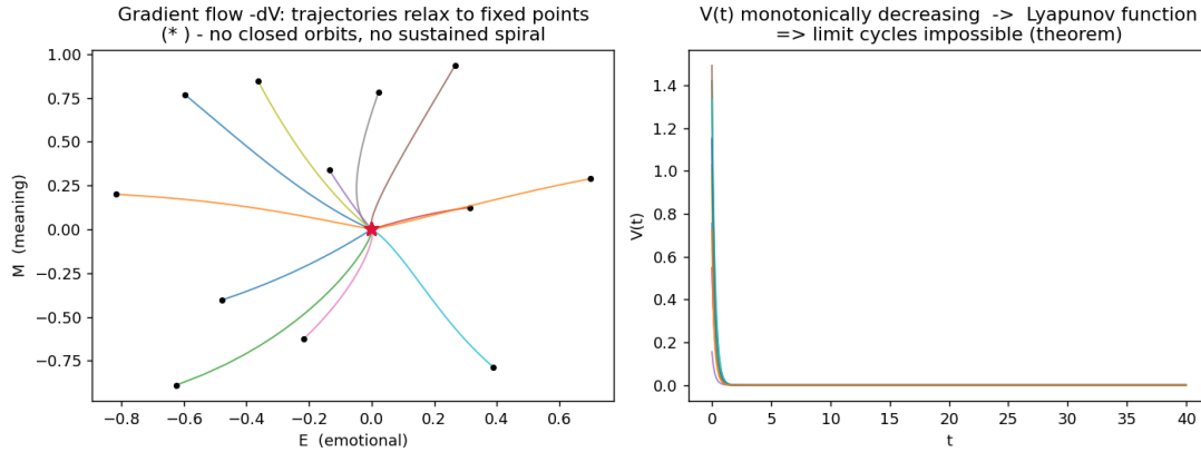
Figure S.3: Gradient flow with the paper's DLHR potentials: trajectories relax to fixed points (no closed orbits, no sustained spiral) and V(t) decreases monotonically, so limit cycles are impossible.
