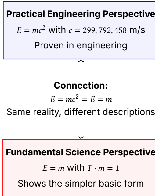
Figure ae.1: The double perspective of T0 Theory
