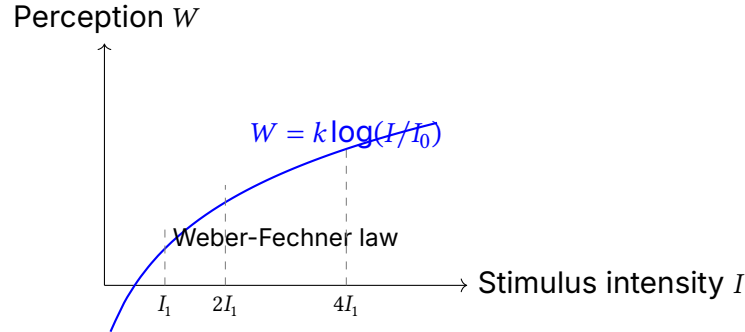
Figure V.1: Logarithmic perception corresponds to the structure of relational systems
