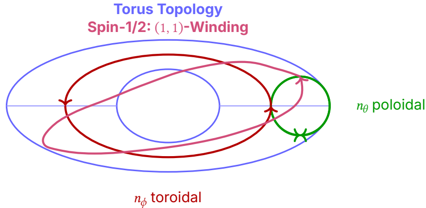
Figure al.1: Spin-1/2 as topological winding on a torus (top view). The green double arrow shows the poloidal small circle ( n_\theta , cross-section of the torus tube). The red arrows show the toroidal direction ( n_\phi , around the central hole). The violet path shows a (1, 1)-winding: once around the small circle AND once around the large circle. A 720^\circ rotation corresponds to traversing this winding twice.
