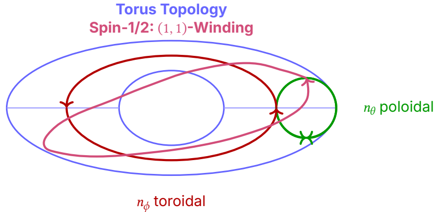
Figure al.1: Spin-1/2 as topological winding on a torus (top view). The green double arrow shows the poloidal small circle ( n_{\theta} , cross-section of the torus tube). The red arrows show the toroidal direction ( n_{\phi} , around the central hole). The violet path shows a (1,1)-winding: once around the small circle AND once around the large circle. A 720^\circ rotation corresponds to traversing this winding twice.
