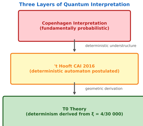
Figure Q.1: Three layers of quantum interpretation: Copenhagen (probabilistic), CAI by 't Hooft (automaton postulated), T0 theory (determinism derived from \xi ). Each level subsumes the previous one.
