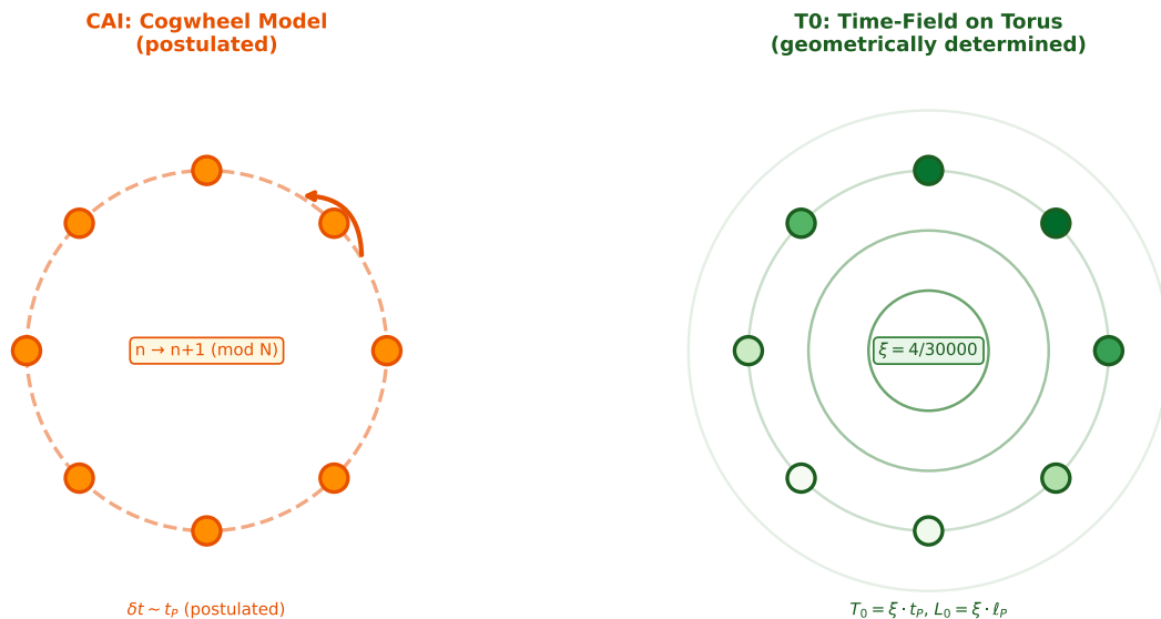
Figure Q.2: Left: CAI cogwheel with N = 8 discrete states (postulated). Right: T0 time field on geometric torus, lattice spacing L_0 = \xi \cdot \ell_p (derived).
