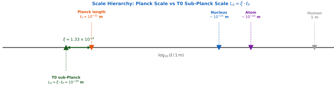
Figure Q.5: Scale hierarchy from human scale to the T0 sub-Planck scale. The T0 lattice constant L_0 = \xi \cdot \ell_P lies by factor \xi \approx 1.33 \times 10^{-4} below the Planck length.
