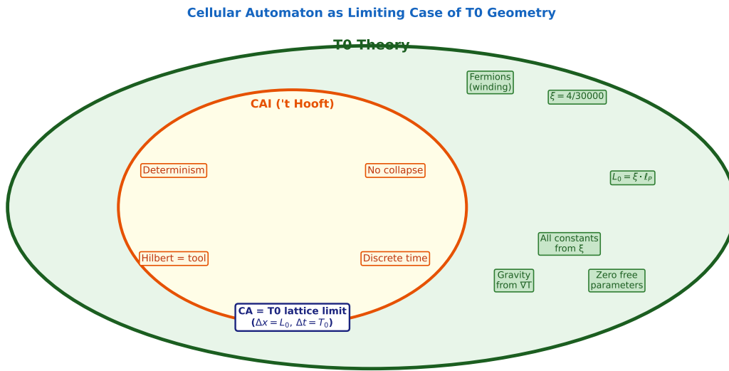
Figure Q.3: Inclusion diagram: the CAI (orange) is contained as a limiting case within T0 theory (green). Outer green elements are T0 contributions beyond the CAI.
