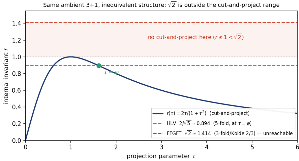
Figure T.1: The cut-and-project invariant r(\tau) \leq 1 reaches HLV's 2/\sqrt{5} at \tau = \varphi but never FFGFT's \sqrt{2} . That \sqrt{2} lies above this family's maximum means only that this particular projection does not interconvert the two invariants – not that the structures are incompatible (see next section).
