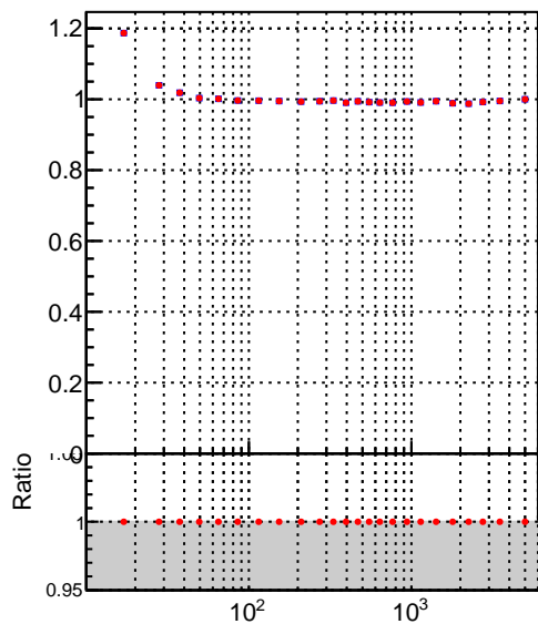
Jet pT response, eta=[0, 1.3]
