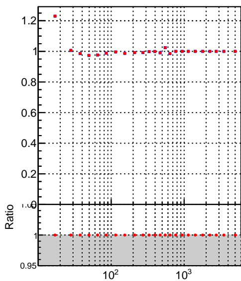
Jet pT response, eta=[2.5, 3.0]
