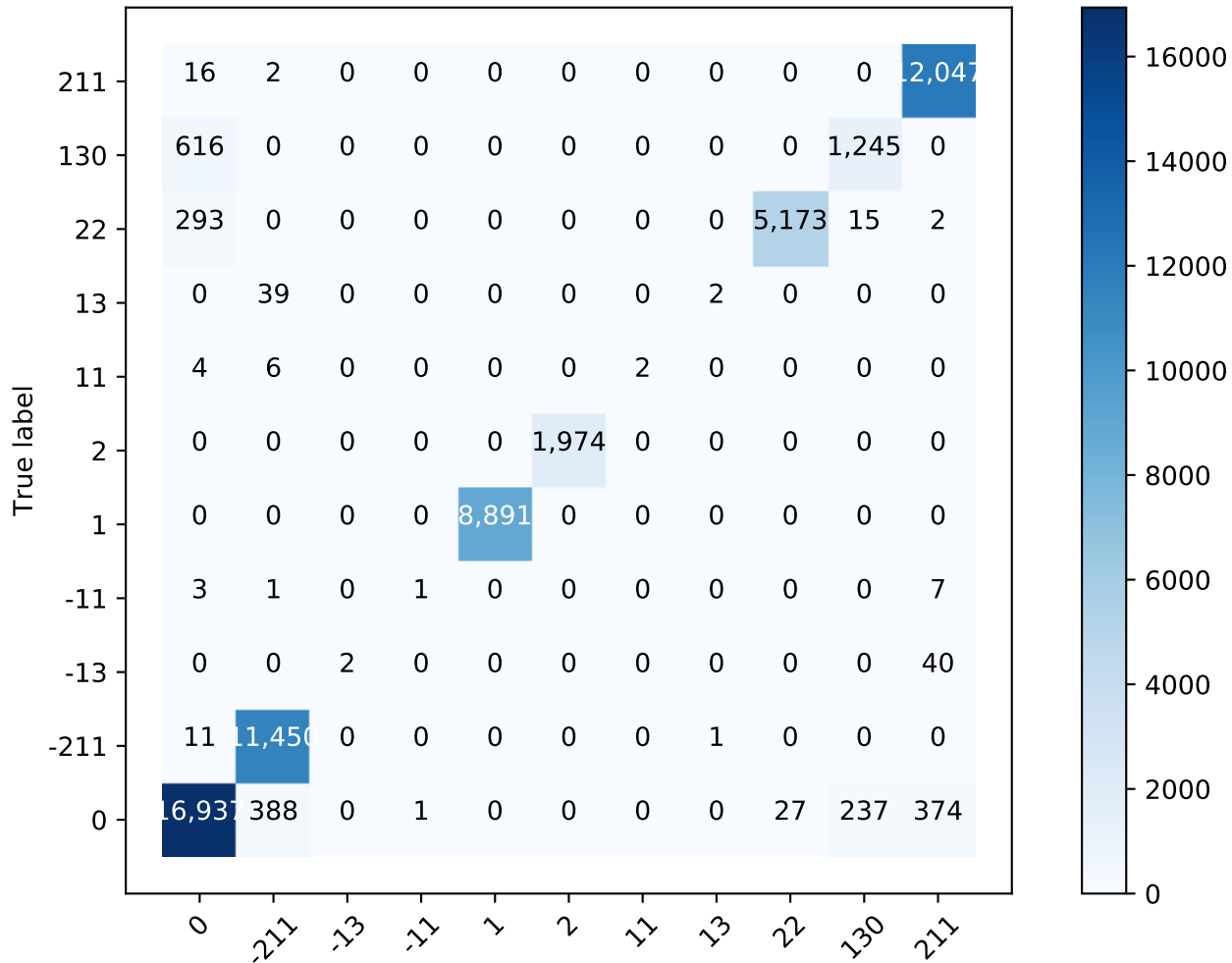
Confusion matrix
