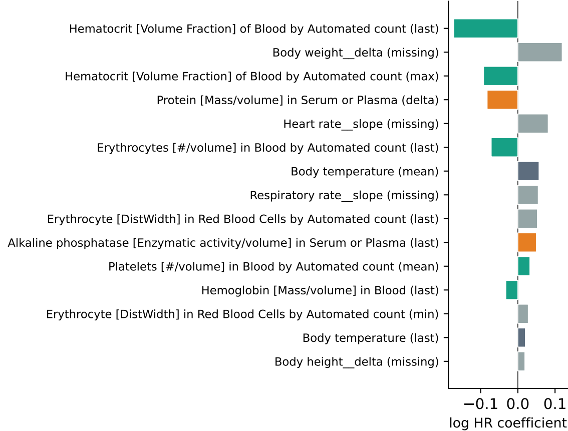
XGBoost Survival · 0 days
