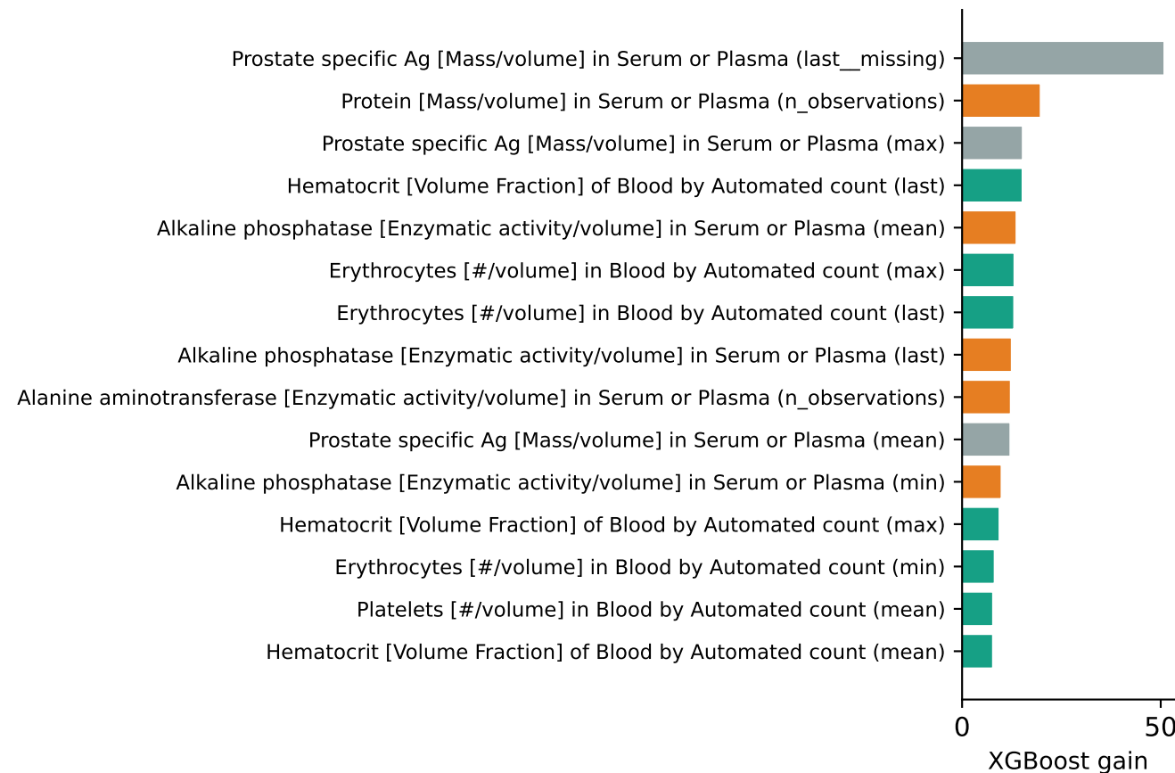
XGBoost Survival · 0 days
