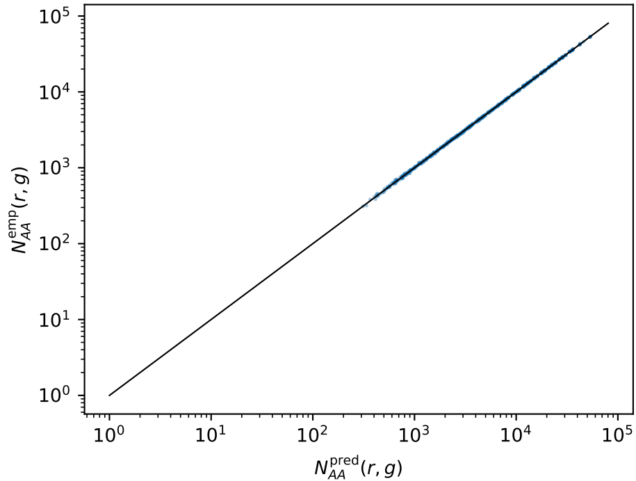
Base 10, 3146 channels mod 840, x = 10^9
