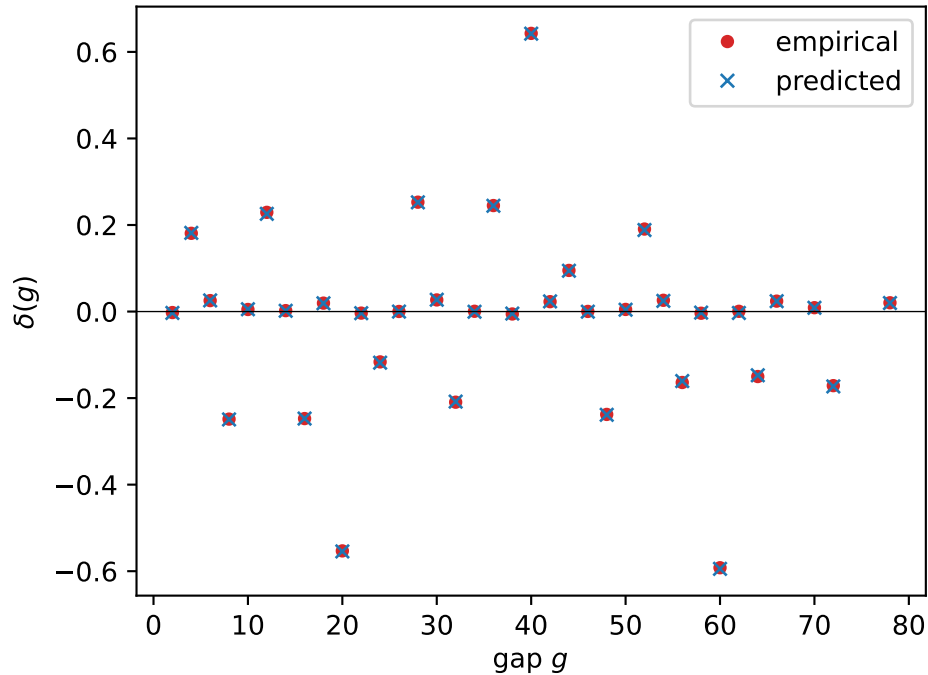
\delta(g) : model vs data, base 10
