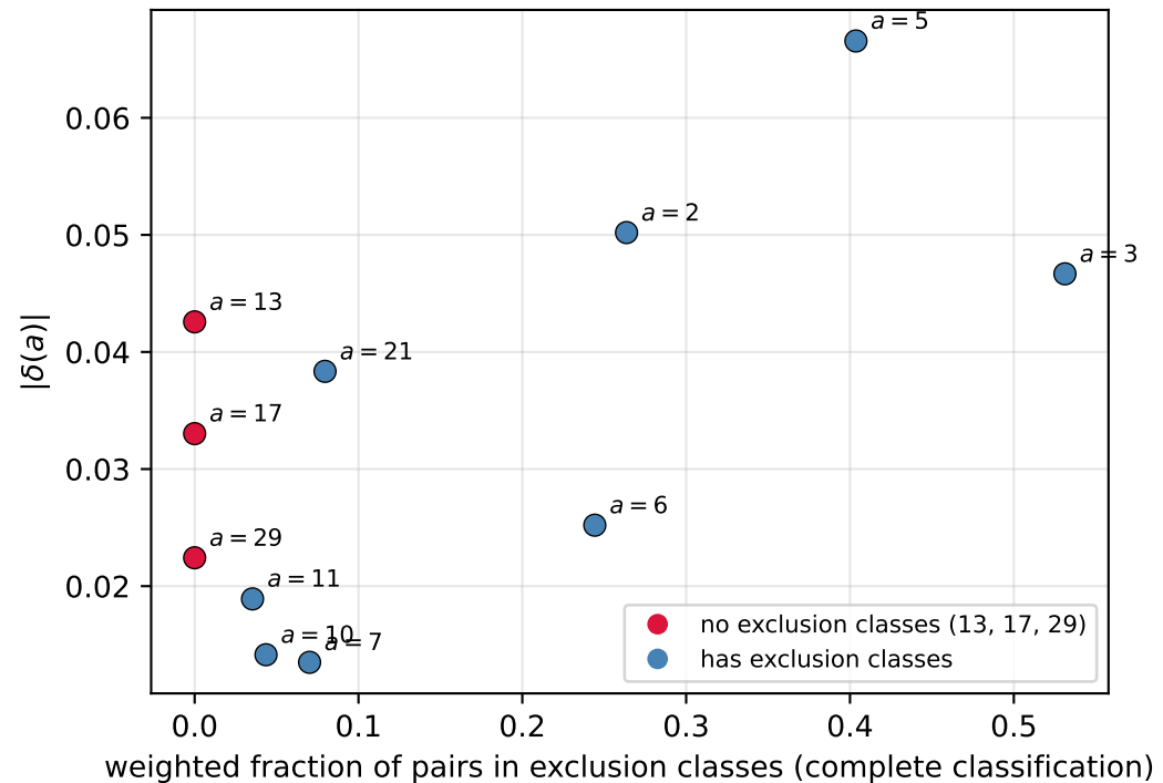
(b) association with exclusion weight is confounded ( r = 0.65 , partial)
