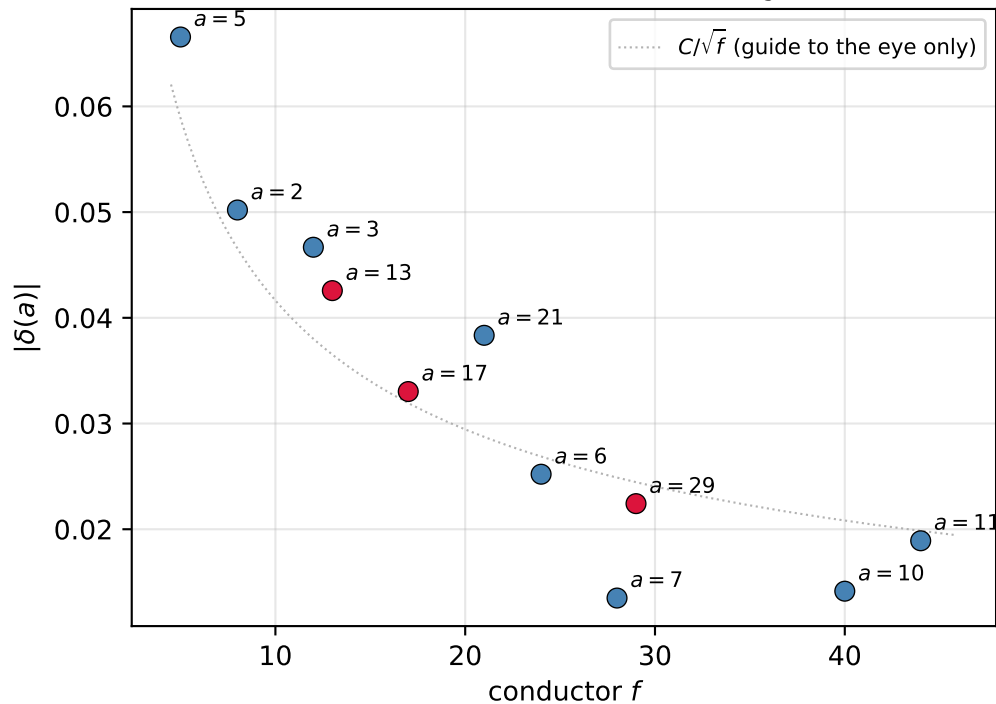
(a) |\delta| decreases with conductor ( r_{\log f} = -0.96 )
