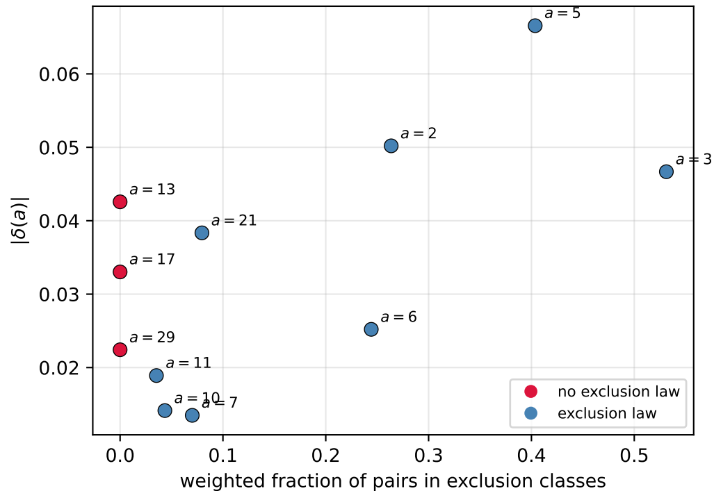
(b) exclusion density: r = 0.65 , but r = 0.14 after adjusting for low
