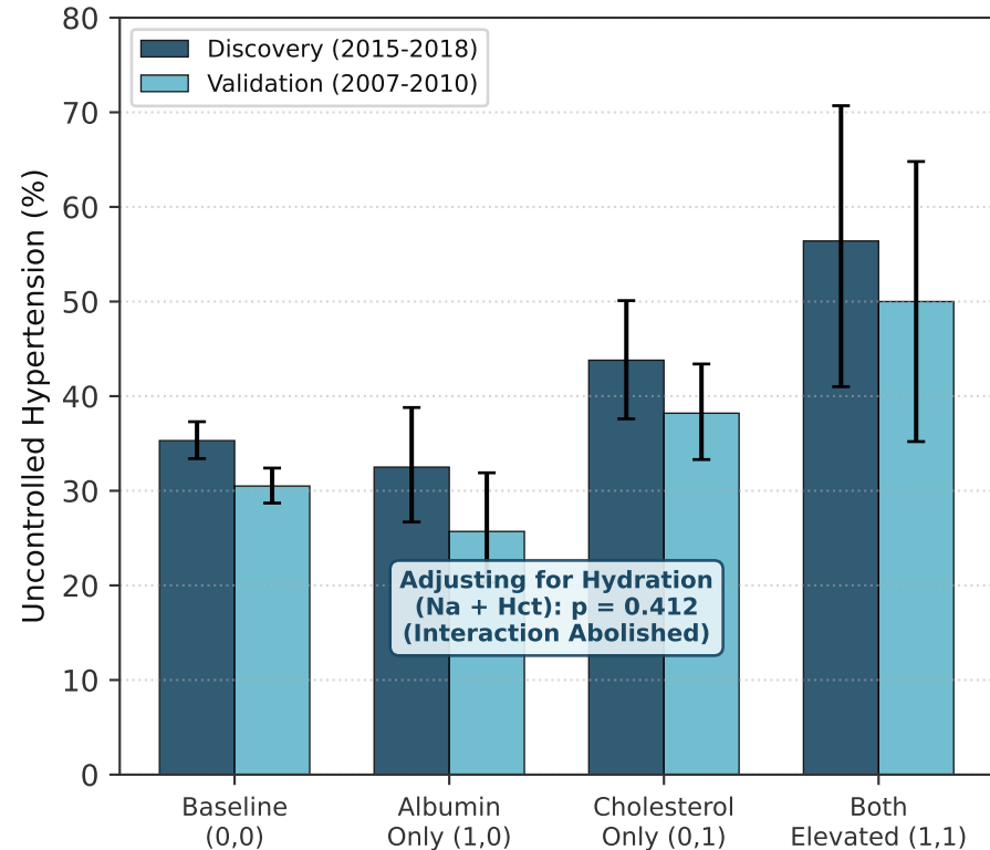
A. Hemoconcentration Trap (Albumin × Cholesterol on HTN)
