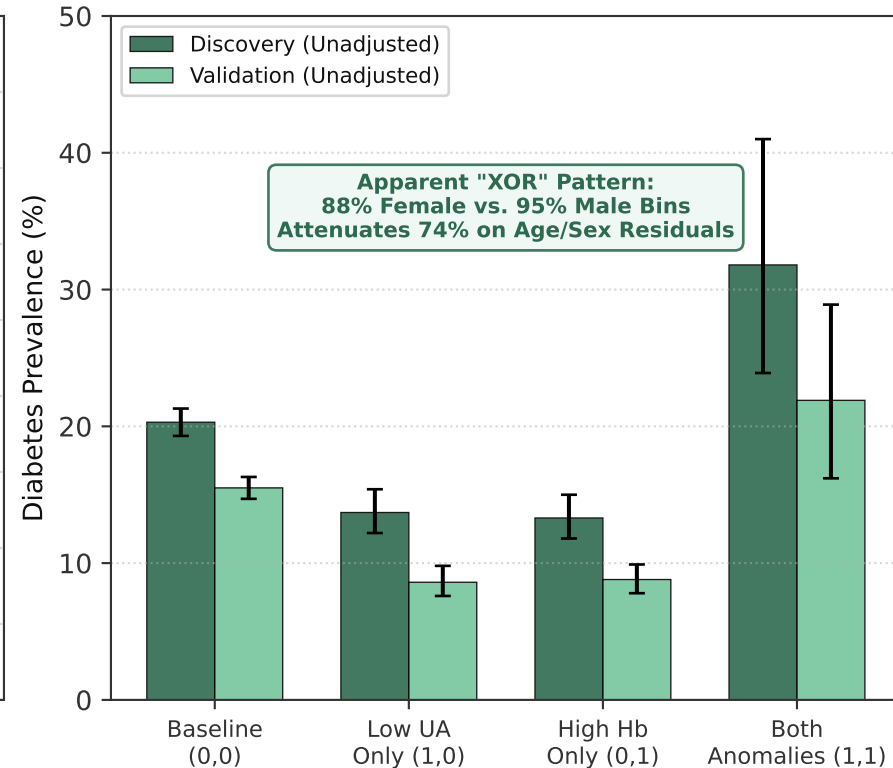
C. Demographic Range Trap (Uric Acid × Hb on Diabetes)
