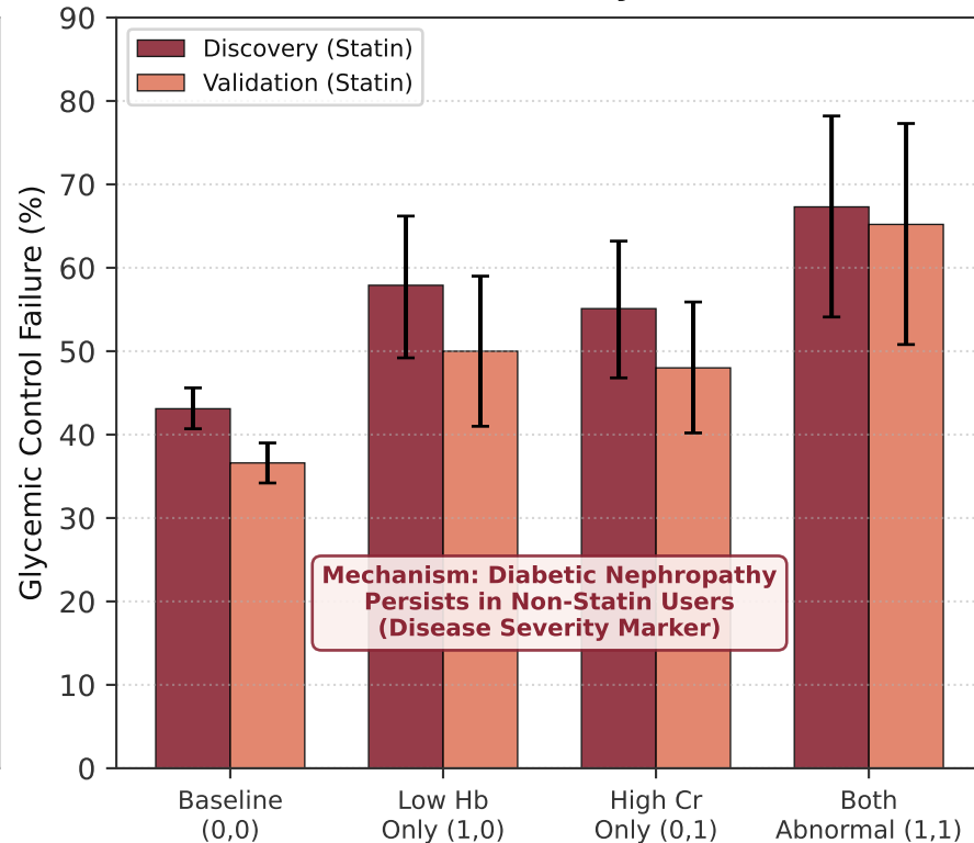
B. Confounding by Indication (Hb × Creatinine on Glycemic Failure)
