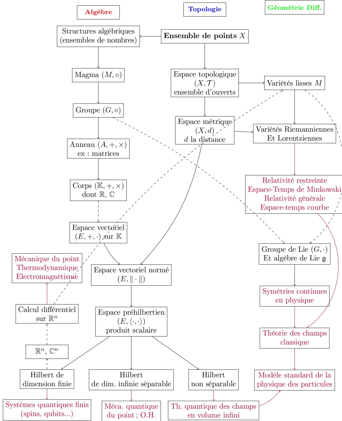
Figure 1.1: An illustrated guide to some mathematical structures used in fundamental physics. Solid black edges from A \rightarrow B indicate that B is a substructure or subset (depending on the case) of A . Dashed edges indicate that the notion A is required to construct B . Arrows and text in purple are reserved for applications to physics. The right branch of differential geometry is not immediately needed in elementary quantum mechanics.
