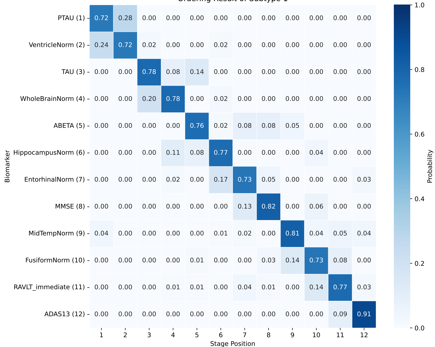
Ordering Result of Subtype 1
