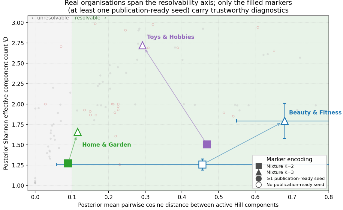
Figure 7: Posterior Shannon effective component count versus posterior mean pairwise cosine distance. The 90 synthetic resolvability fits form a faint backdrop (grey filled = converged, open salmon = non-converged). The three real organisations (averaged across seeds, error bars \pm 1 s.d.) are foregrounded by colour, with marker shape encoding K (square = K=2 , triangle = K=3 ) and fill encoding diagnostic trust: a filled marker had at least one publication-ready seed, a hollow marker none. A thin arrow joins each organisation’s K=2 and K=3 fits. The shaded region right of the dashed line ( \bar{d}_{\text{cos}} \approx 0.10 ) is the resolvable side of the transition identified in Section 5.2.
