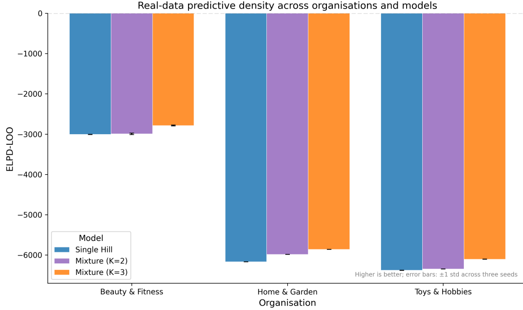
Figure 8: Real-data ELPD-LOO across the three organisations and three models. Higher is better. Error bars are \pm 1 standard deviation across three NUTS reruns at different random seeds and represent Monte Carlo variability of the sampler, not data-level uncertainty; in particular they should not be read as paired se_diff between models. Mixture K = 3 has the highest estimated mean ELPD-LOO in every organisation, subject to the paired-SE and PSIS reliability caveats above.
