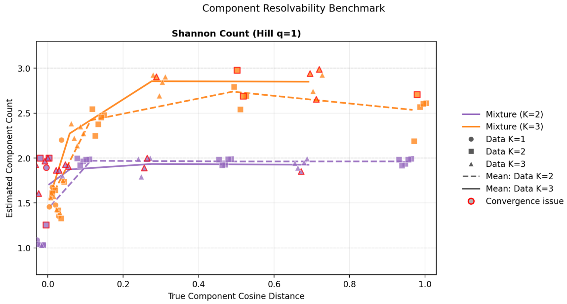
Figure 6: Component resolvability: Shannon effective count of the posterior versus mean pairwise cosine distance of the true Hill curves. Red-outlined points indicate cases that failed the publication-ready convergence criterion.
