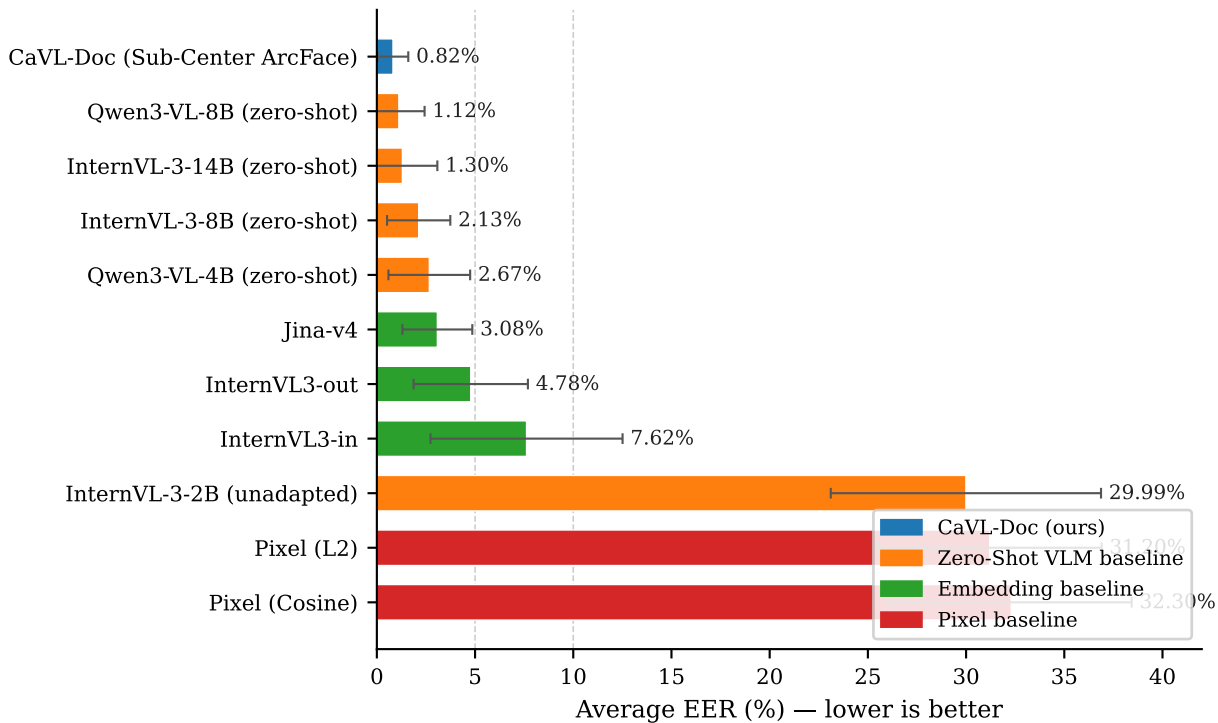
Method Comparison on LA-CDIP (Avg. EER, Splits 0-4)
