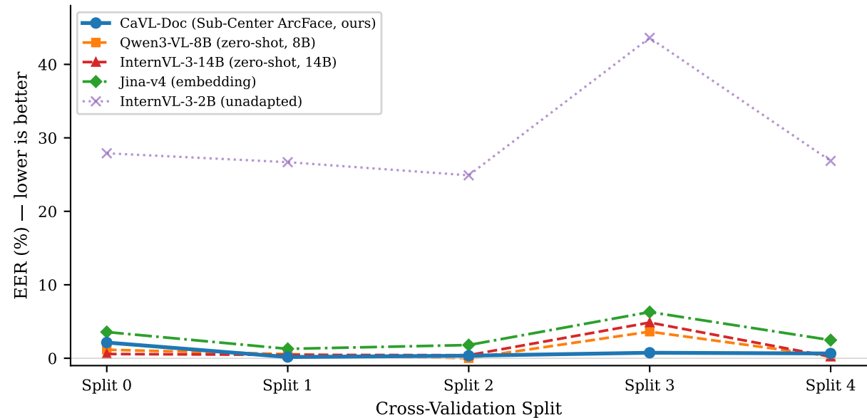
Per-Split EER Breakdown on LA-CDIP
