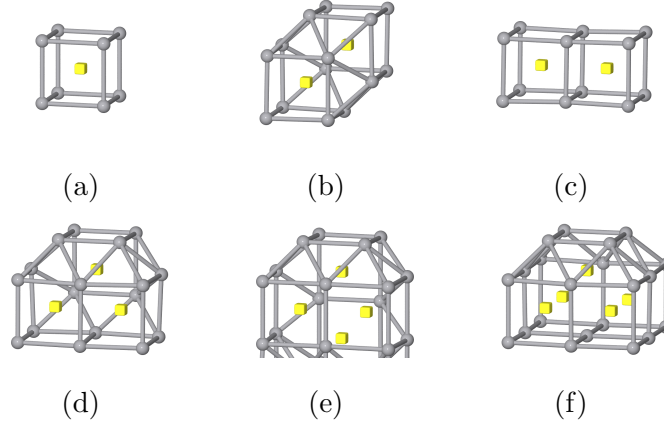
Figure 1: Lowest formation energy vacancy type clusters V_m . (a) V_1 , (b) V_2(1nn) , (c) V_2(2nn) , (d) V_3 , (e) V_4 , (f) V_5 . Vacancies are represented with yellow cubes.
