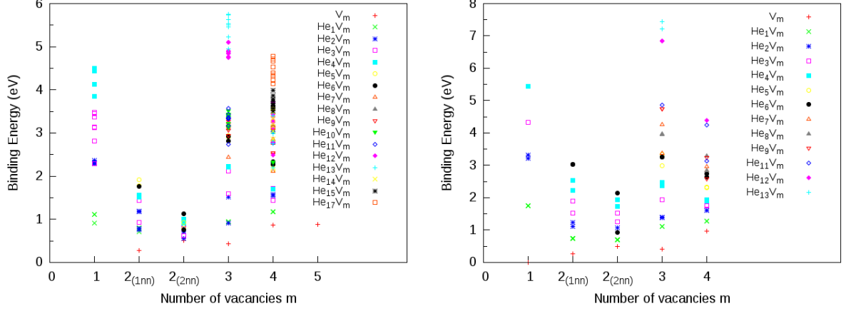
Figure 6: Binding energy of mono-vacancy to He n V m clusters as a function of m in vanadium (left panel) and tantalum (right panel)
