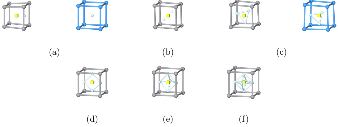
Figure 2: Lowest formation energy \text{He}_n \text{V}_1 type clusters in vanadium and tantalum. (a) \text{He}_1 \text{V}_1 , (b) \text{He}_2 \text{V}_1 , (c) \text{He}_3 \text{V}_1 , (d) \text{He}_4 \text{V}_1 , (e) \text{He}_5 \text{V}_1 , (f) \text{He}_6 \text{V}_1 . Vacancy is represented with yellow cube, vanadium with grey ball, tantalum with dark blue ball and helium with light blue ball. Configurations for tantalum are shown only when different to vanadium ones.
