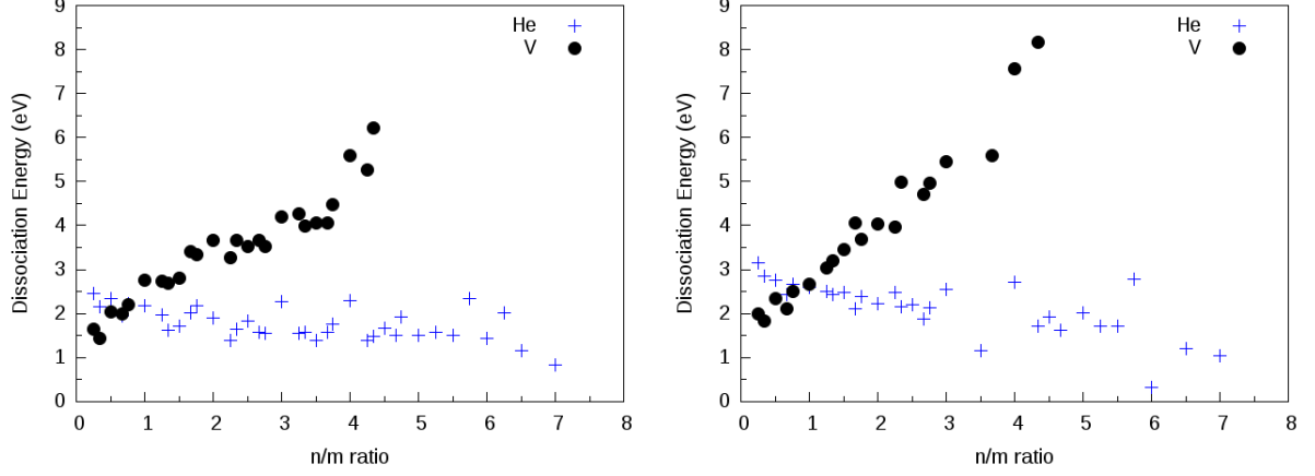
Figure 7: Dissociation energy of He and vacancy to \text{He}_n\text{V}_m as a function of n/m ratio for the most stable clusters in vanadium (left panel) and tantalum (right panel).
