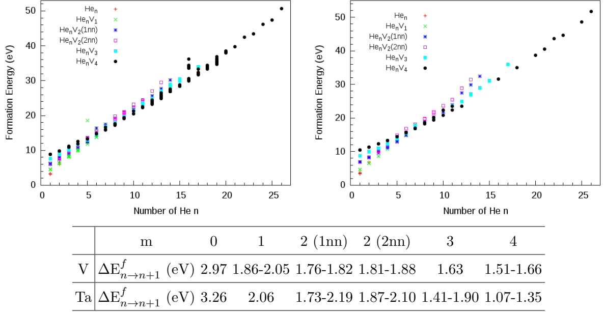
Figure 4: Formation energy as a function of n in vanadium (left panel) and tantalum (right panel). For di-vacancy clusters the label (1nn) is for 1st vacancy nearest neighbour and (2nn) for 2nd nearest vacancy neighbour. The table gives the slope for each type of cluster.
