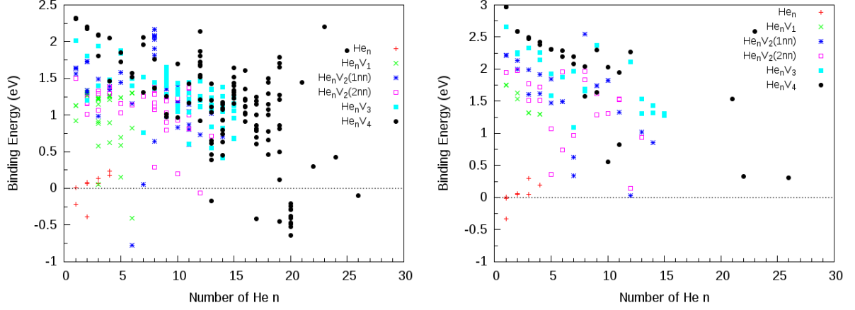
Figure 5: Binding energy of He to He n V m clusters as a function of n in vanadium (left panel) and tantalum (right panel)
