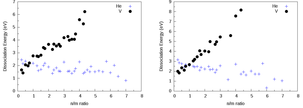
Figure 8: Dissociation energy of He and vacancy to \text{He}_n\text{V}_m as a function of n/m ratio for the most stable clusters in vanadium (left panel) and tantalum (right panel).
