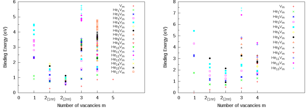
Figure 7: Binding energy of mono-vacancy to He n V m clusters as a function of m in vanadium (left panel) and tantalum (right panel)
