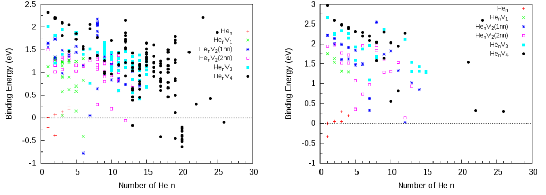
Figure 6: Binding energy of He to \text{He}_n\text{V}_m clusters as a function of n in vanadium (left panel) and tantalum (right panel)
