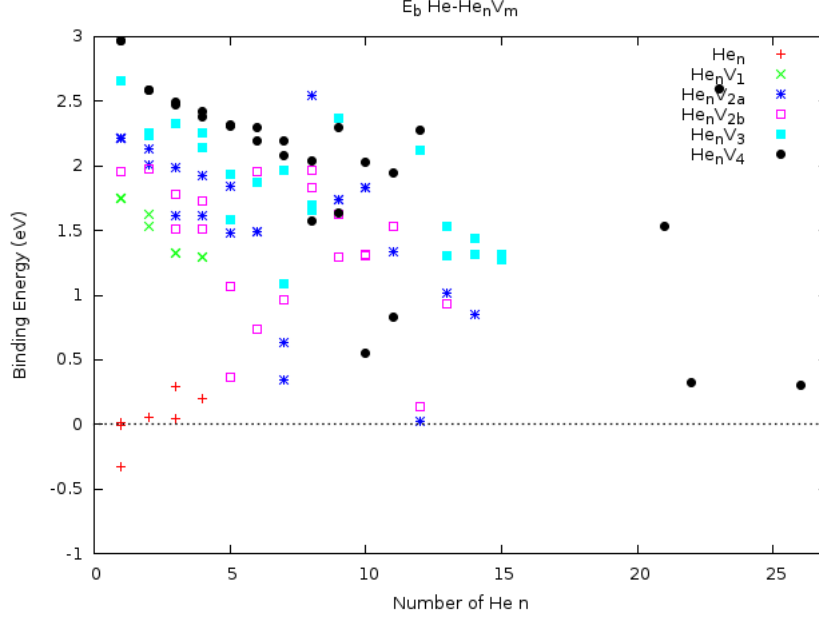
Figure 9: Binding energy of He to \text{He}_n \text{V}_m clusters as a function of n in tantalum
