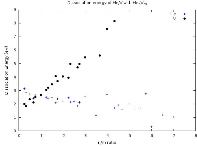
Figure 13: Dissociation energy of He and vacancy to \text{He}_n\text{V}_m as a function of n/m ratio for the most stable clusters in tantalum.
