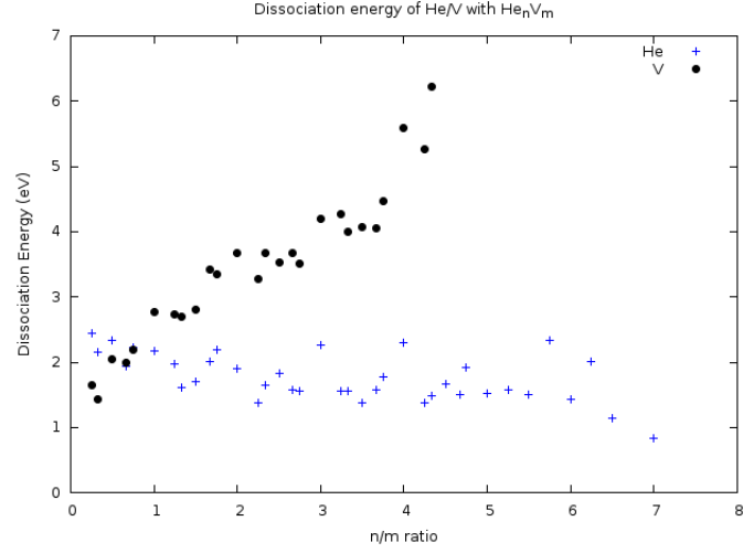
Figure 12: Dissociation energy of He and vacancy to \text{He}_n\text{V}_m as a function of n/m ratio for the most stable clusters in vanadium.
