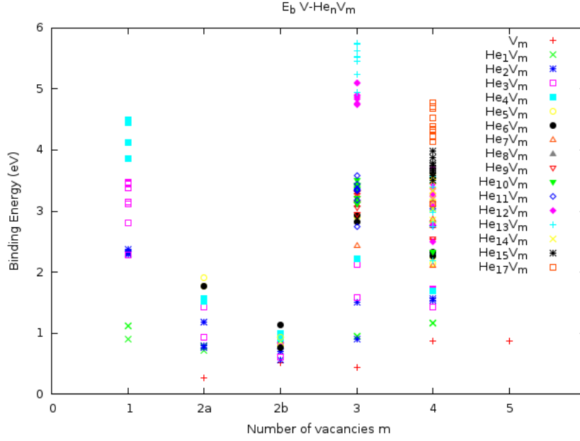
Figure 10: Binding energy of mono-vacancy to \text{He}_n \text{V}_m clusters as a function of m in vanadium
