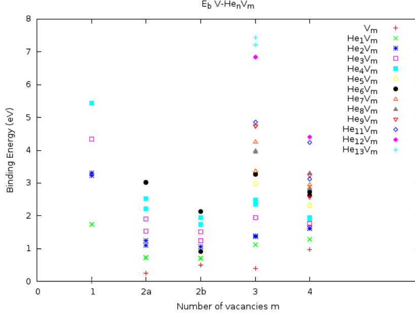
Figure 11: Binding energy of mono-vacancy to \text{He}_n\text{V}_m clusters as a function of m in tantalum
