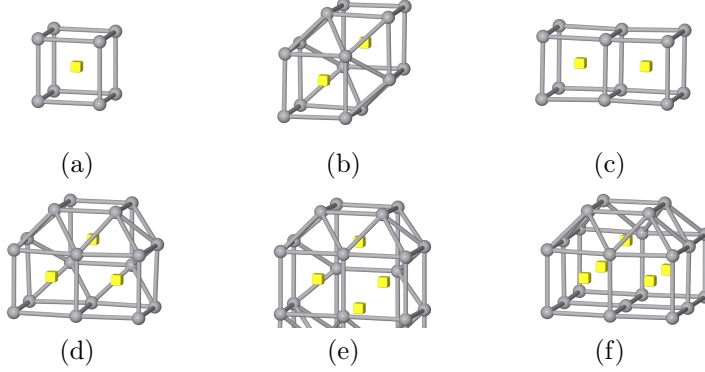
Figure 1: Lowest formation energy vacancy type clusters V_m . (a) V_1 , (b) V_{2a} , (c) V_{2b} , (d) V_3 , (e) V_4 , (f) V_5 . Vacancies are represented with yellow cubes.
