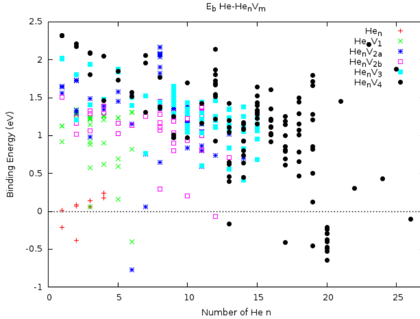
Figure 8: Binding energy of He to \text{He}_n\text{V}_m clusters as a function of n in vanadium
