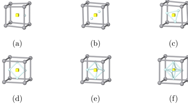
Figure 2: Lowest formation energy \text{He}_n V_1 type clusters in vanadium. (a) \text{He}_1 V_1 , (b) \text{He}_2 V_1 , (c) \text{He}_3 V_1 , (d) \text{He}_4 V_1 , (e) \text{He}_5 V_1 , (f) \text{He}_6 V_1 . Vacancy is represented with yellow cubes and He atoms with light blue balls.
