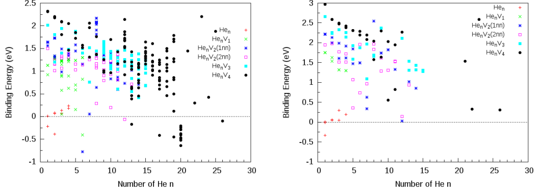
Figure 5: Binding energy of He to He n V m clusters as a function of n in vanadium (left panel) and tantalum (right panel)
