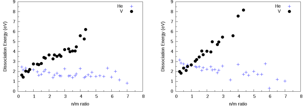
Figure 7: Dissociation energy of He and vacancy to \text{He}_n\text{V}_m as a function of n/m ratio for the most stable clusters in vanadium (left panel) and tantalum (right panel).
