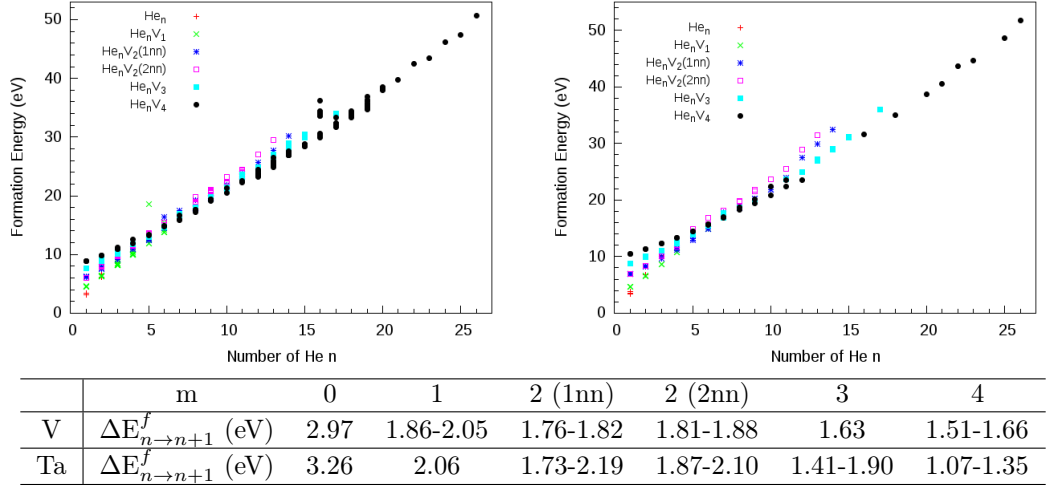
Figure 4: Formation energy as a function of n in vanadium (left panel) and tantalum (right panel). For di-vacancy clusters the label (1nn) is for 1st vacancy nearest neighbour and (2nn) for 2nd nearest vacancy neighbour. The table gives the slope for each type of cluster.
