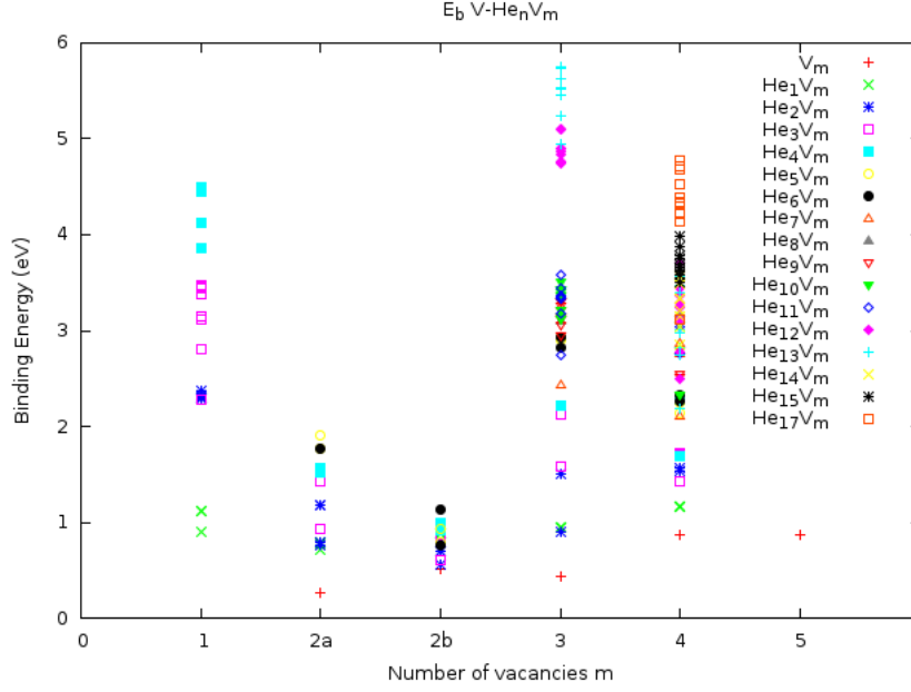
Figure 8: Binding energy of mono-vacancy to \text{He}_n \text{V}_m clusters as a function of m in vanadium
