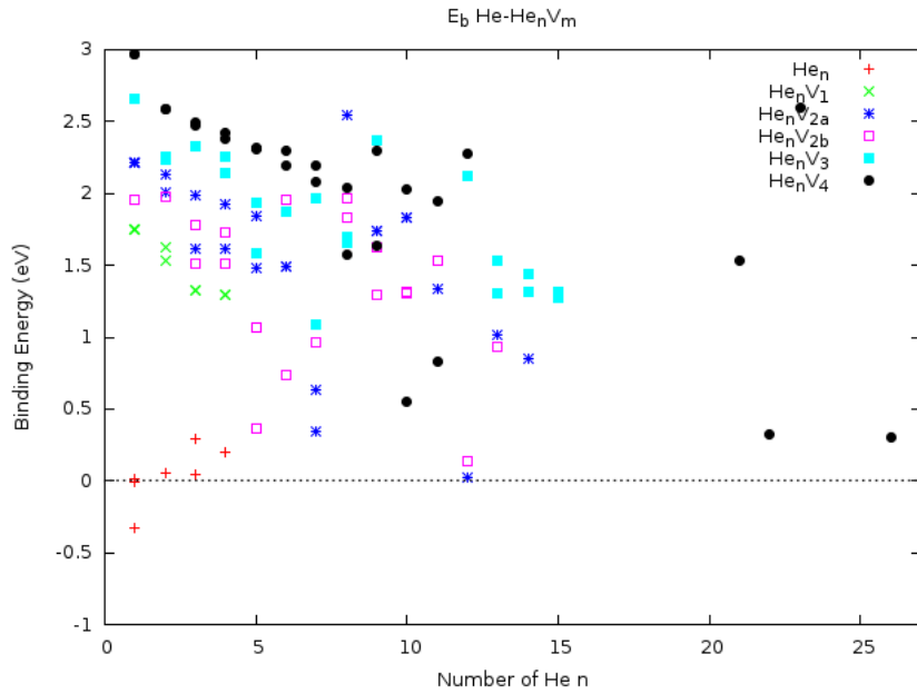
Figure 7: Binding energy of He to He n V m clusters as a function of n in tantalum
