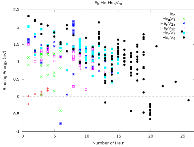
Figure 6: Binding energy of He to He n V m clusters as a function of n in vanadium
