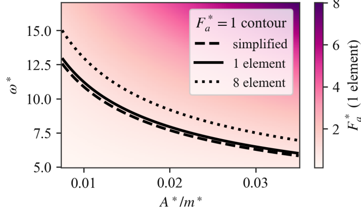
Figure 3: Verification of F_a^* = 1 contour at reference condition
