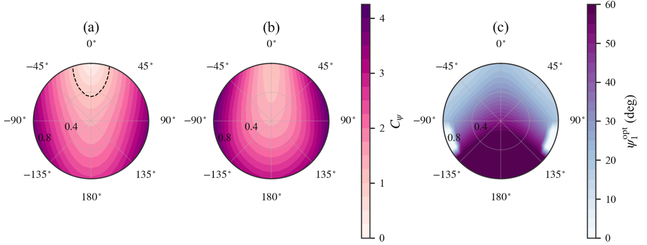
Figure 13: C_\psi over the body-velocity plane (radius: advance ratio J , angle: \chi from the stroke-plane normal), at \psi_0 = 0 , \delta_0 = 90^\circ , for the reference configuration. (a) Hover-optimal pitch ( \psi_1 = 51^\circ ), dashed line marks C_\psi = 1 . (b) \psi_1 re-optimized at each velocity over the range of Table 1. (c) The re-optimized \psi_1 .
