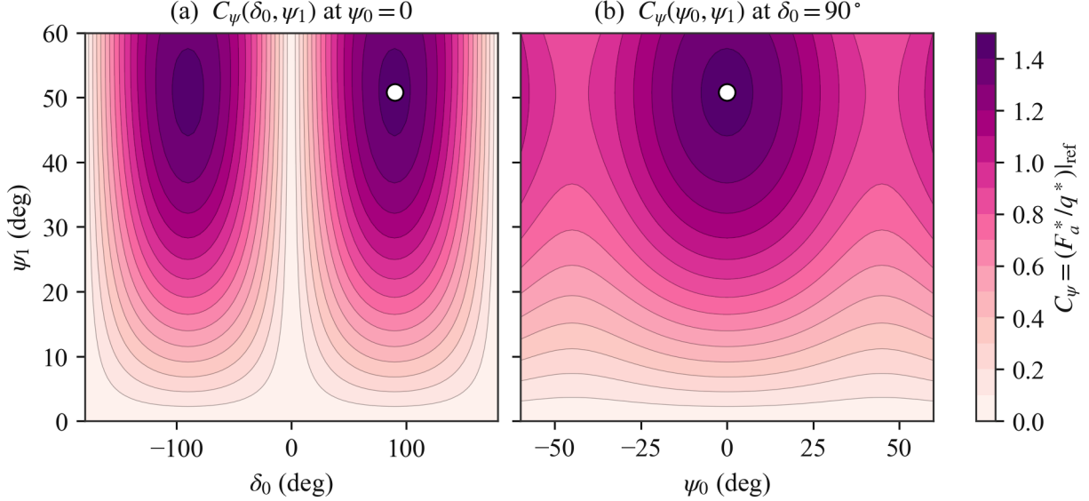
Figure 5: Dependence of C_\psi on pitch parameters at zero body velocity. Optimal value shown as white dots.
