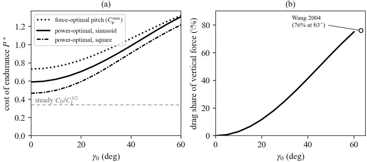
Figure 8: Hover power efficiency vs. stroke-plane angle, reference configuration. (a) Cost of endurance P^* for the force-optimal (maximum- C_\psi ) pitch and for the power-optimal pitch with a sinusoidal and a square-wave feather, all re-trimmed to hover at each \gamma_0 ; the steady-flight ideal C_D/C_L^{3/2} is shown for reference. (b) Share of the cycle-averaged vertical force carried by drag rather than lift, with the result of [1] marked.
