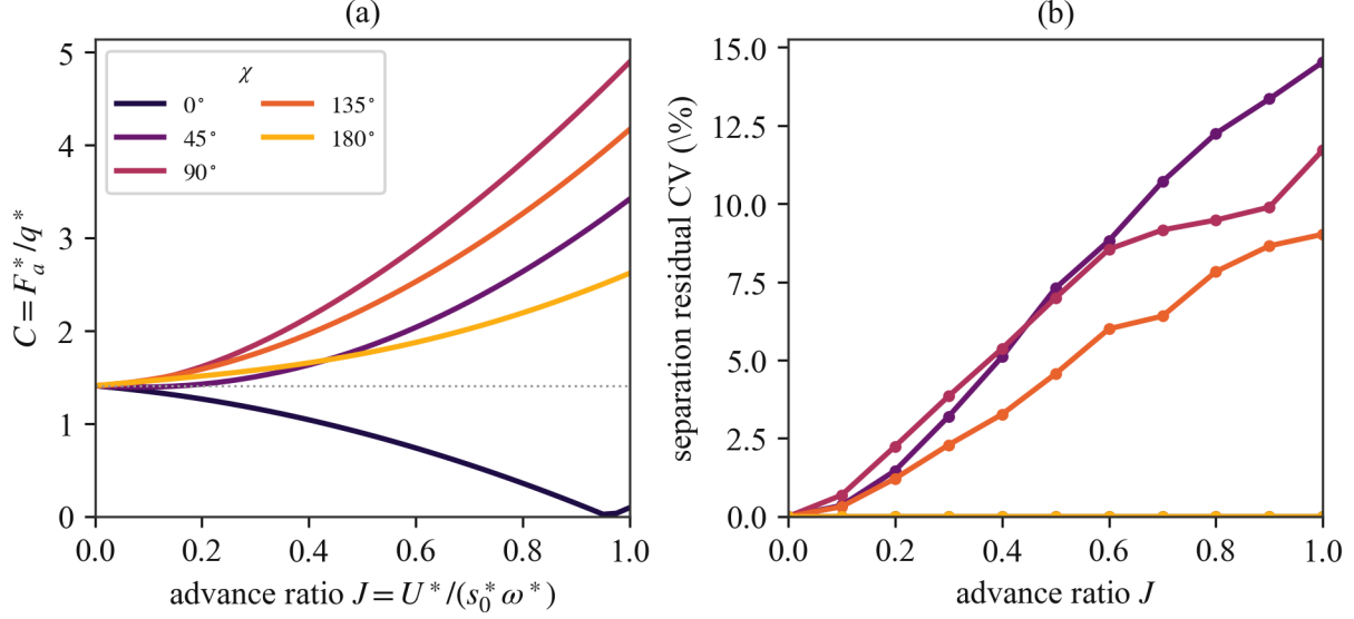
Figure 12: Survival of the F_a^* = q^* C_\psi separation at nonzero body velocity. (a) C_\psi at nominal pitch as a function of advance ratio for several inflow directions \chi . (b) Separation residual, evaluated as the coefficient of variation of F_a^* / q^* over random draws of the morphological and wingbeat parameters at fixed pitch.
