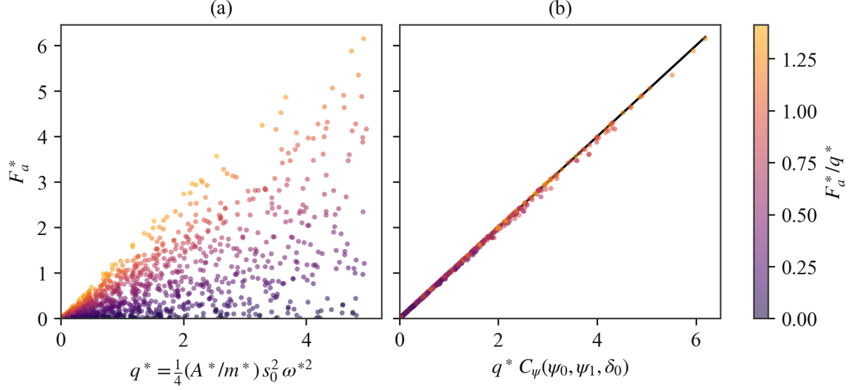
Figure 4: Separation of dynamic pressure and wing pitch factors of the aerodynamic force at zero body velocity. (a) Scatter of mean aerodynamic force as a function of dynamic pressure for random sampling of parameter space (b) Collapse of scatter by introduction of C_\psi parameter evaluated as F_a^*/q^* for a reference amplitude value s_0^* = 0.25
