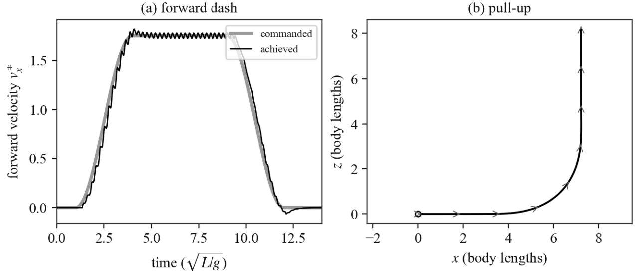
Figure 15: Closed-loop maneuvers (unsteady simulation, control updated once per wingbeat). (a) Forward dash: commanded vs. achieved forward velocity through accelerate–cruise–decelerate. (b) Pull-up: the sagittal-plane path, with body-velocity arrows rotating from horizontal to vertical.
