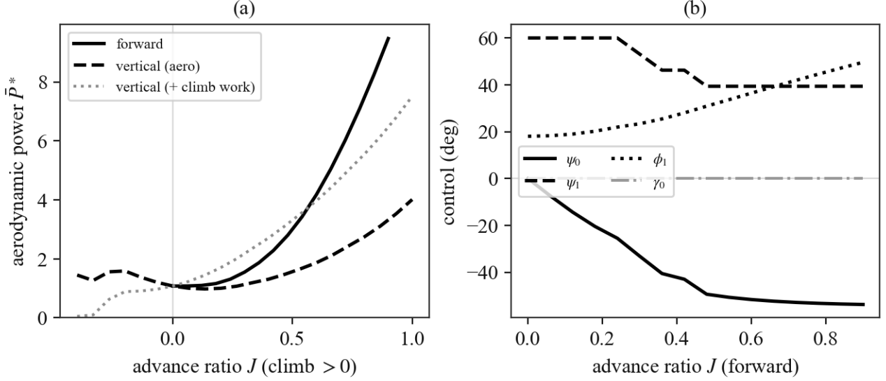
Figure 14: Power-optimal straight-flight trim vs. body velocity, reference configuration. (a) Aerodynamic power \bar{P}^* vs. advance ratio for forward and vertical flight; the dotted curve adds the climb work V_z W to the vertical aerodynamic power to give the metabolic cost. (b) The forward-flight control schedule: \psi_0 steers (and saturates), \psi_1 re-tunes down, \phi_1 grows for magnitude, and the power-optimal \gamma_0 stays at zero.
